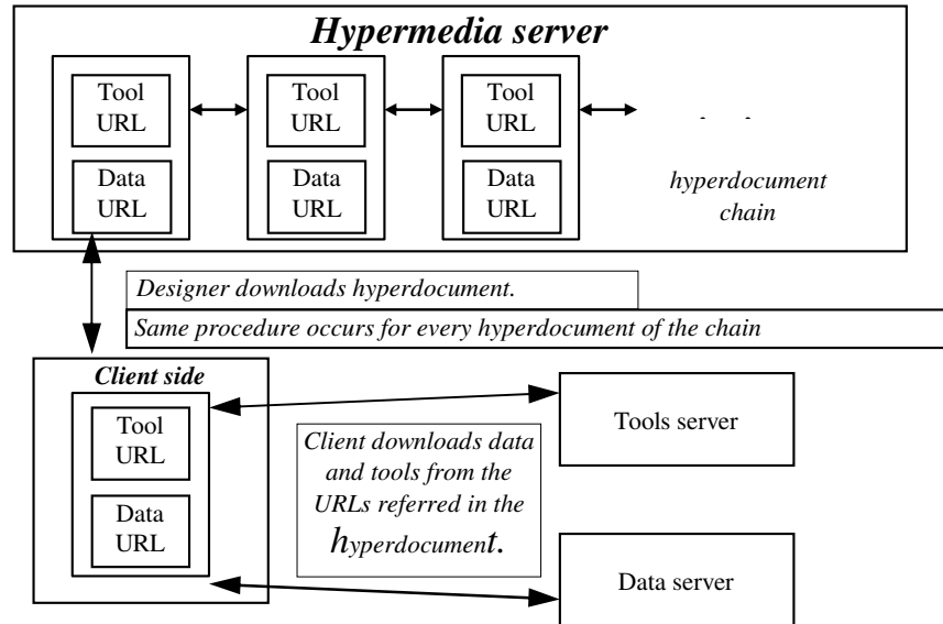
Fig.3.- Tool-tool integration architecture.
